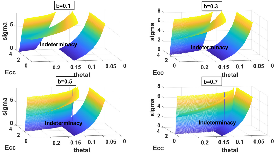
Figure 10: Indeterminacy area for different values of b .
