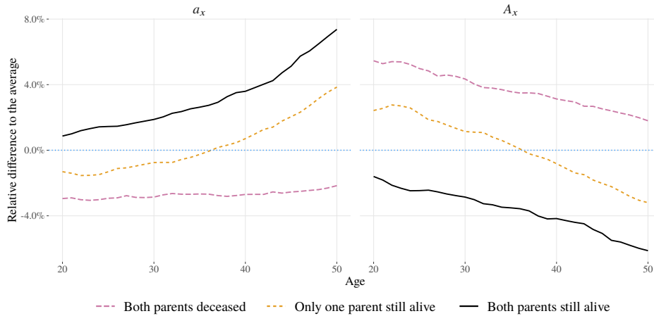
Figure 12. Relative difference to the average (in %) of present value of an annuity (left) and expected present value for a life insurance (right) depending on the age of the annuitant and on how many parents are still alive at the time of the contract.
