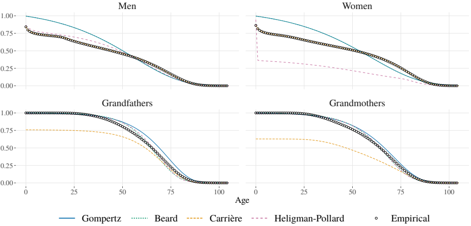
Figure C5. Survival function for individuals depending on their gender (top), and for their grandparents (bottom).
