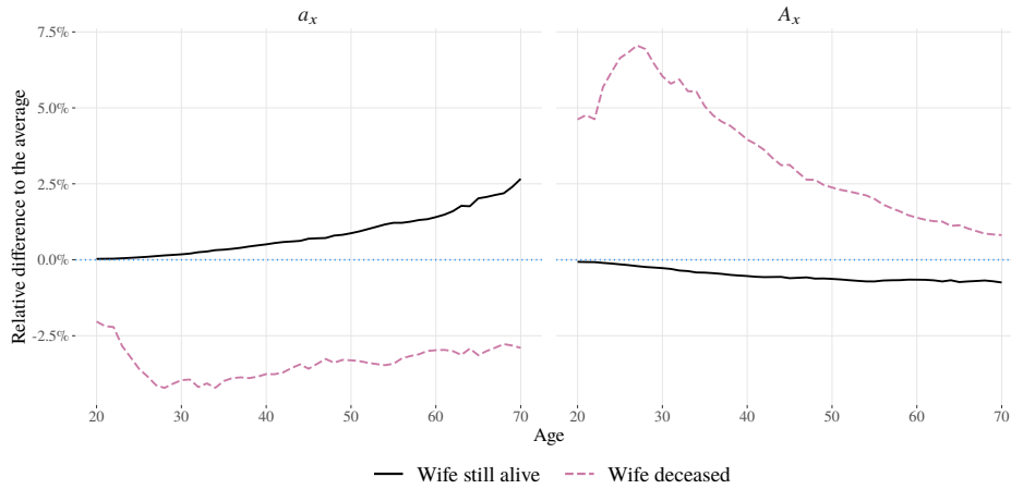
Figure 6. Relative difference to the average (in %) of present value of an annuity (left) and expected present value for a life insurance (right) depending on the age of the annuitant and on the death status of the wife at the time of the contract.
