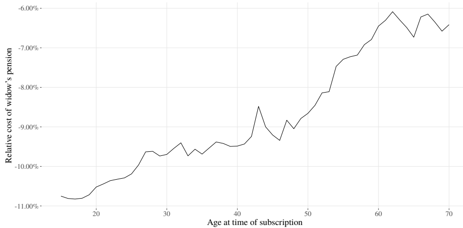
Figure 7. Widow's pension, a_{m|f} (relative to independent case a_{m|f}^+ ), as a function of x_m .
