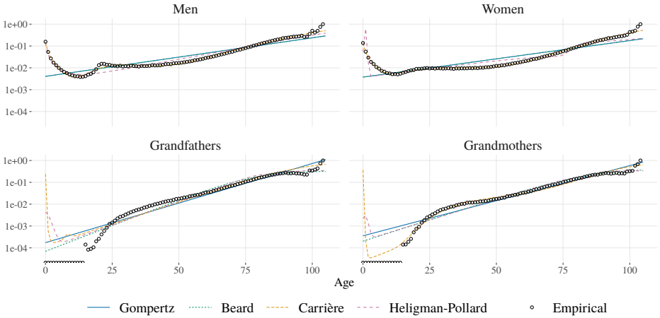
Figure C4. Force of mortality (log scale) \mu_x for individuals depending on their gender (top), and for their grandparents (bottom).
